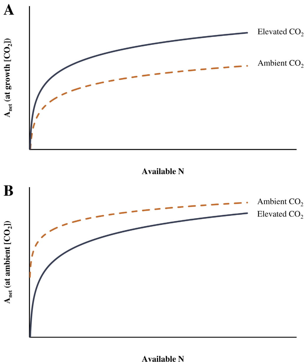
Fig. 2. Photosynthetic response to \text{CO}_2 enrichment and available N. (A) \text{CO}_2 assimilation rate, measured at growth [ \text{CO}_2 ] (ambient or elevated; dashed and solid lines, respectively), as a function of available N. (B) \text{CO}_2 assimilation rate, measured at ambient [ \text{CO}_2 ], as a function of available N. Note, photosynthetic acclimation occurs in plants grown on elevated \text{CO}_2 and is most pronounced under low-N conditions. Redrawn from Wong, 1979 (see also Sage, 1994; Bowler and Press, 1996; Miglietta et al., 1996; Stitt and Krapp, 1999; cf. Farage et al., 1998).
